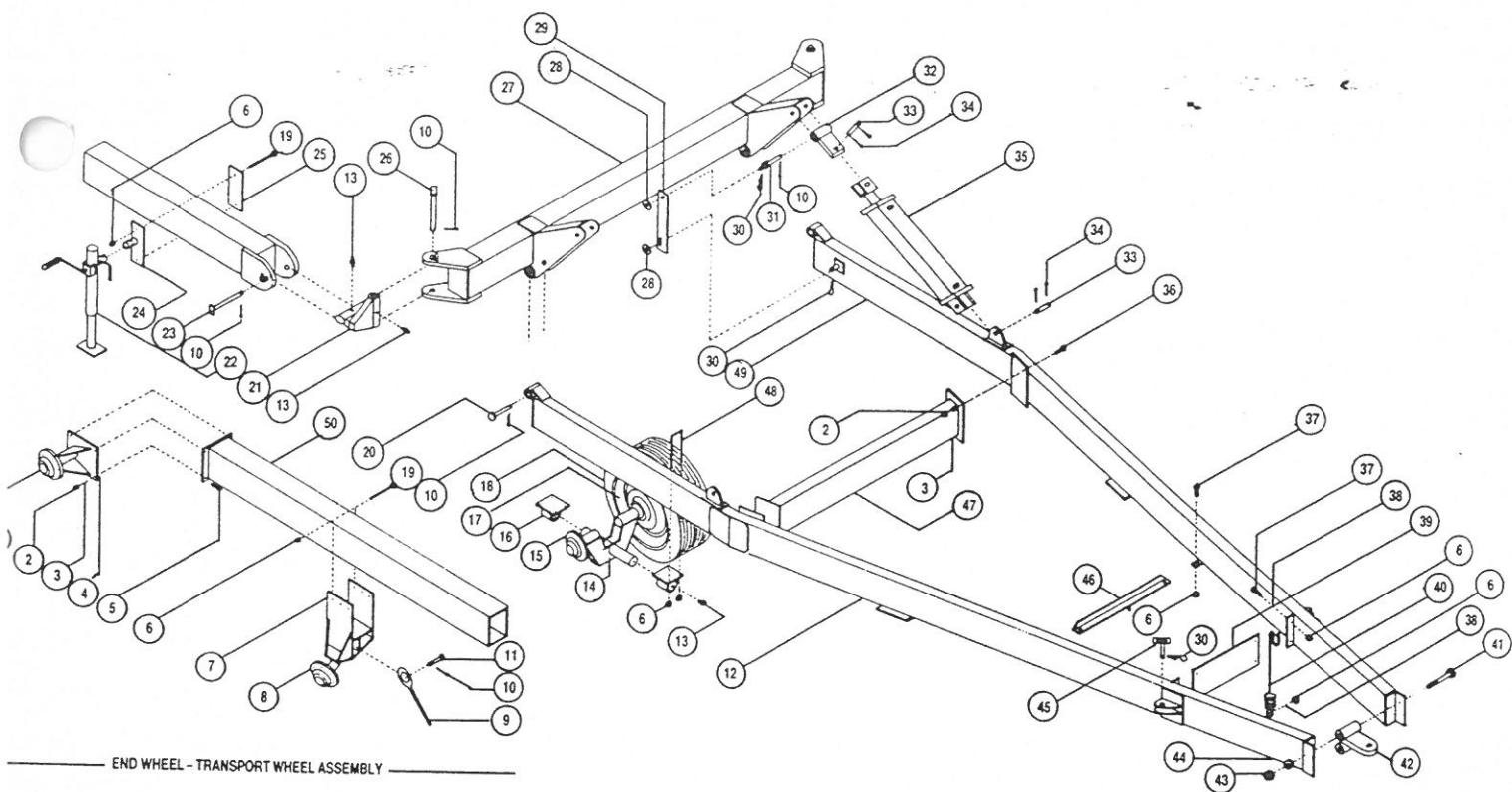
20 FOOT A-FRAME HITCH ASSEMBLY
