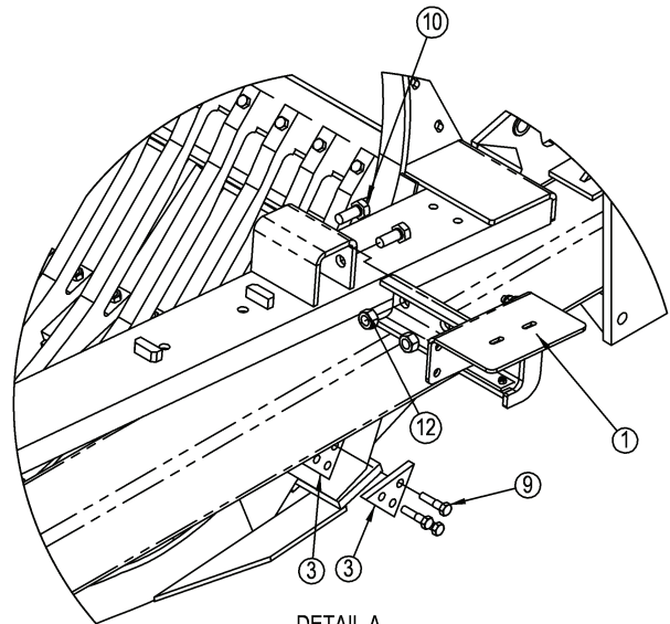
DETAIL A SCALE 1 : 12
