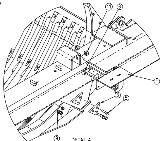
DETAIL A SCALE 1 : 12
