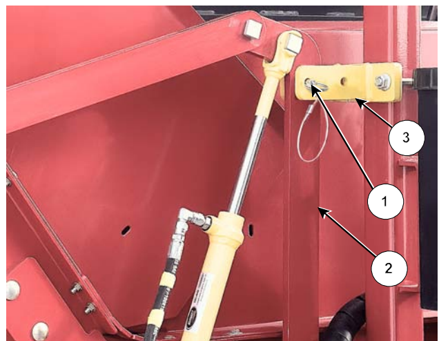
Remove the Flip Conveyor Lock
