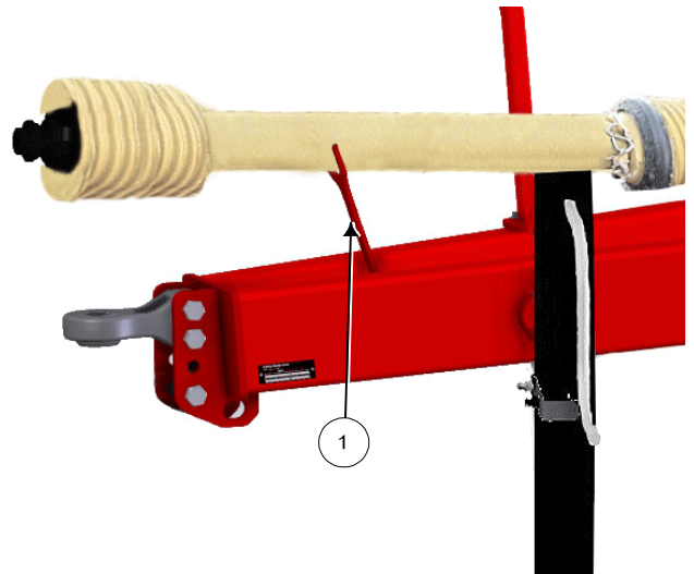
Place the Driveline into the Driveline Support
