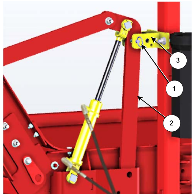
Lock the Flip Conveyor into Transport Position
