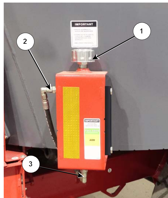
If Tank Has Been Overfilled, Drain Some Oil
