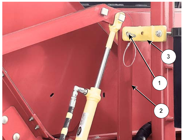
Lock the Flip Conveyor into Transport Position
