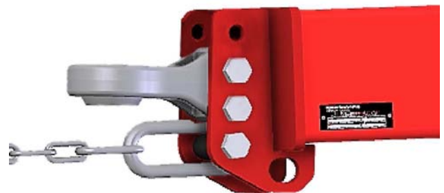
Tongue Set for Tractor Drawbar 17" or Lower from the Ground
