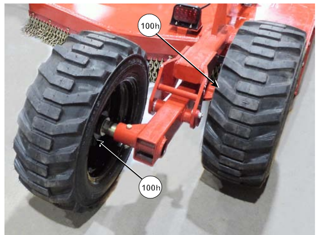
Grease Wing Hubs
