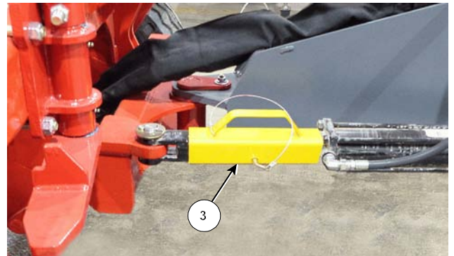
Hitch Cylinder Transport Locks
