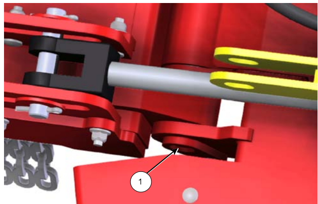
Right Wing Rear Pivot
