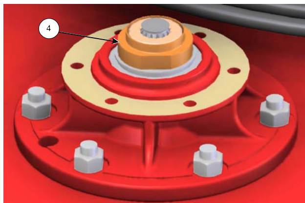
Motor and Adaptor Removed, Shaft Nut Accessible
