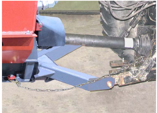
Attach the Driveline to the PTO Adjust 2 Point Connection for Driveline Level
