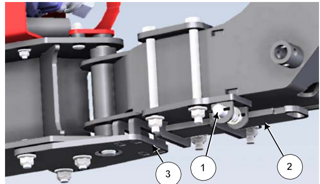
Ensure the Lower Hitch Lock is Removed
