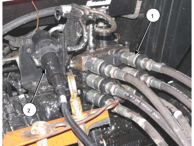
Attach Hydraulics and Lighting (3 Remote Model Connections Shown)
