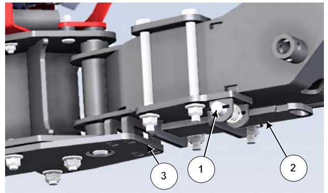
Ensure the Lower Hitch Lock is Removed
