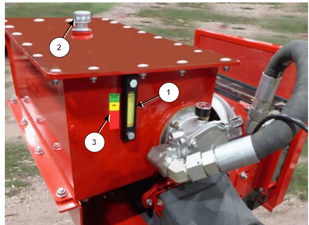
Remove the Breather Cap
