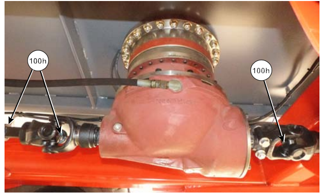
Front Screw Driveline
