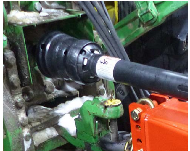
Disconnect the Driveline from the Tractor
