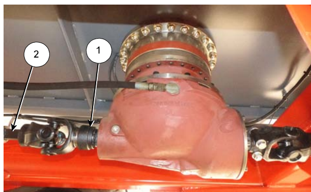
Reconnect the Driveline to the Rear Screw
