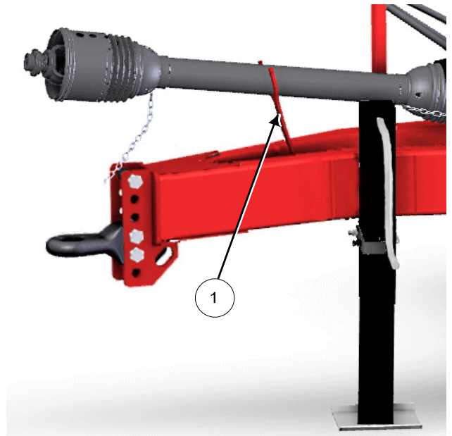
Place the Driveline into the Driveline Support
