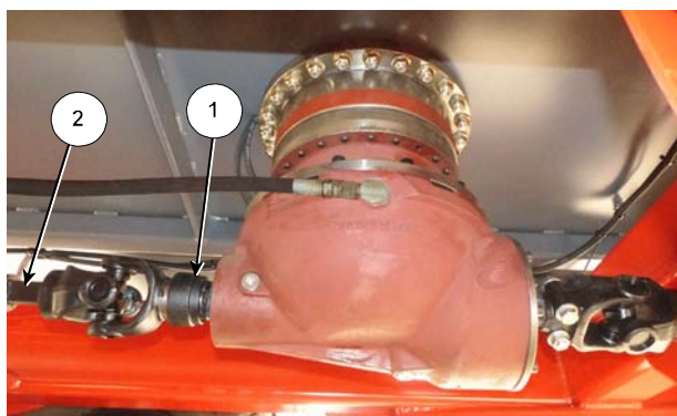
Disconnect Front Screw Driveline
