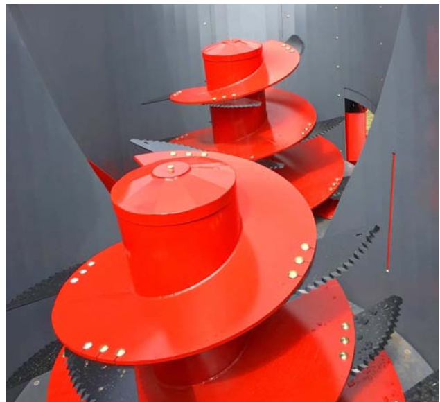
Check the Knives on the Screws
