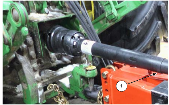
Connect the Driveline to PTO
