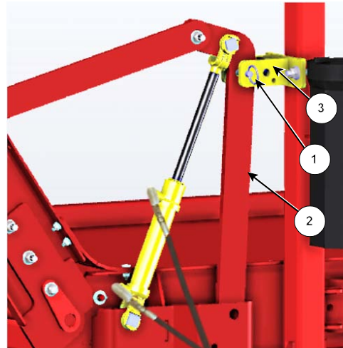
Remove the Flip Conveyor Lock 223235C
