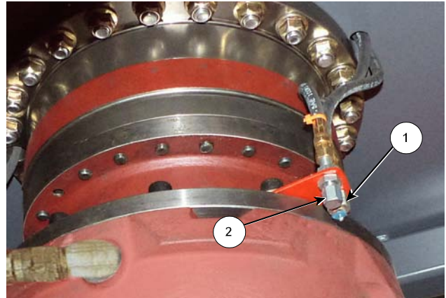
Grease Screw Drivebox Top Bearing
