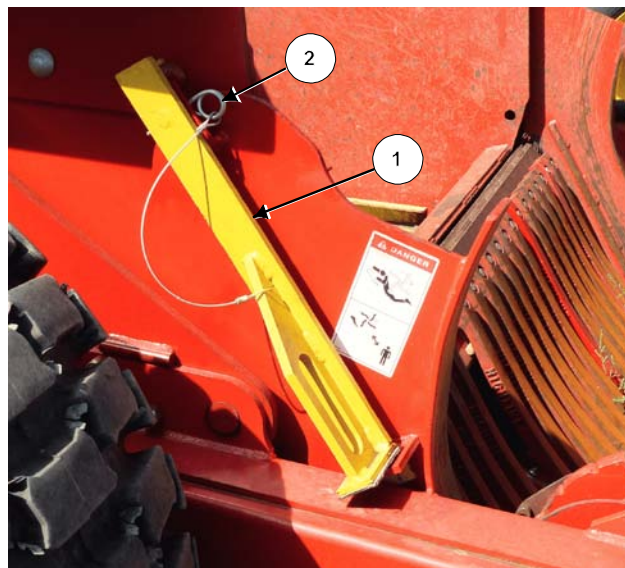
Remove the Right Apron Lock
