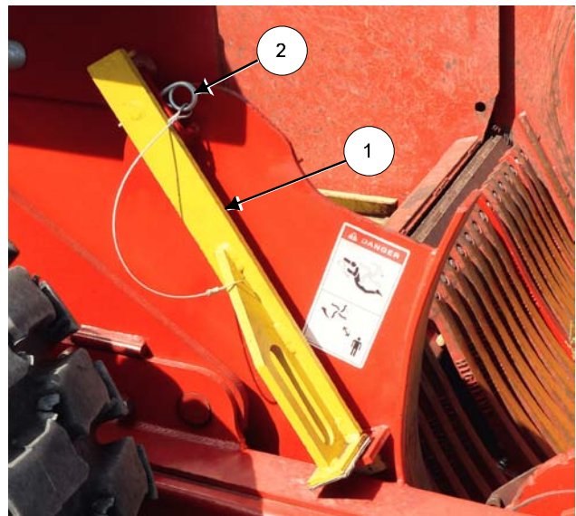
Right Apron Lock in Storage
