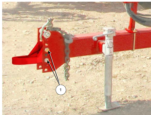
Adjust Tongue to Level the Rockpicker (Regular Tongue Shown)
