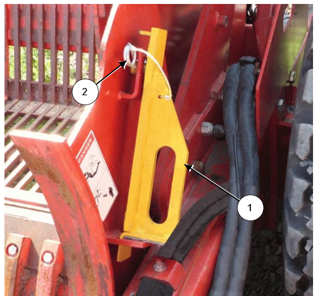
Left Apron Lock in Storage Position
