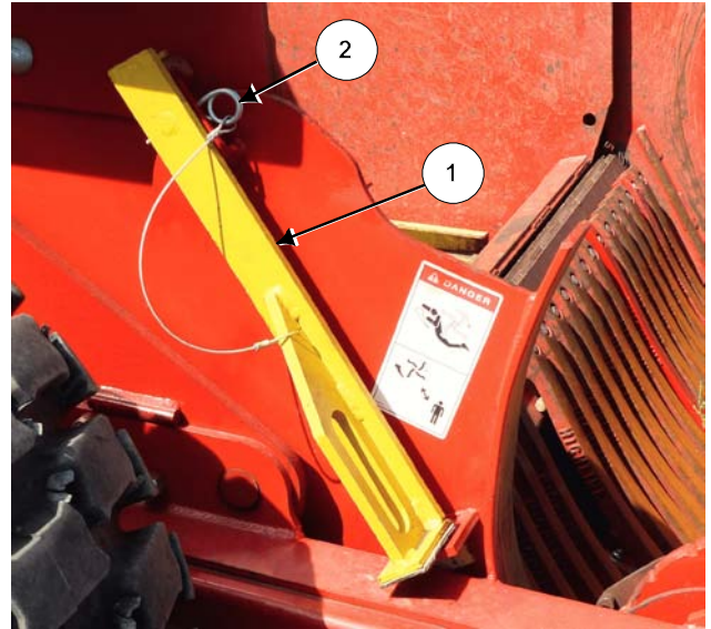
Remove the Right Apron Lock
