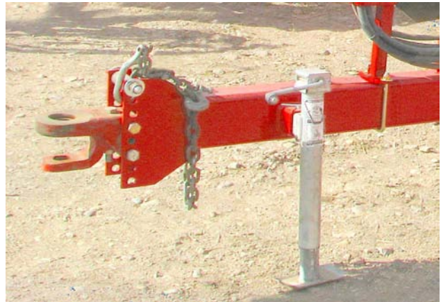
Lift the Hitch with the Jack (Clevis Tongue Shown)
