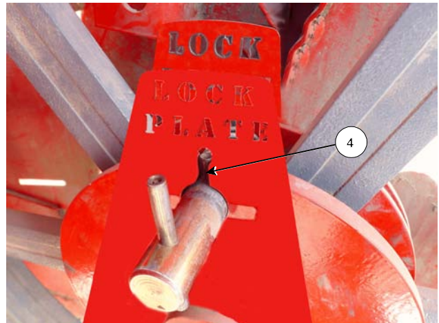
Twist Clutch Pin to Disengage Drive
