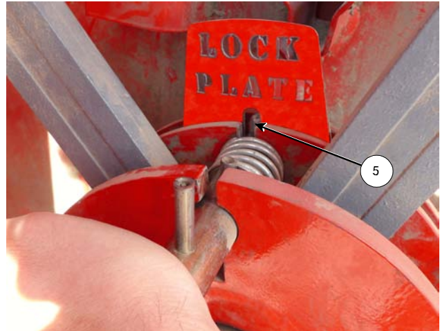
Push and Twist Clutch Pin (Front Lock Plate Not Shown for Clarity)
