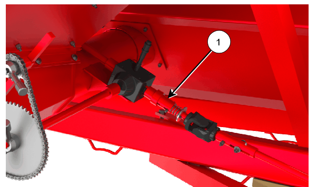
Check The One Way Clutch
