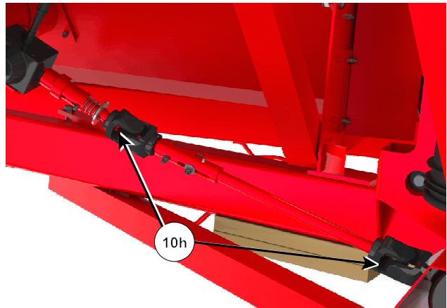
Grease Universal Joints
