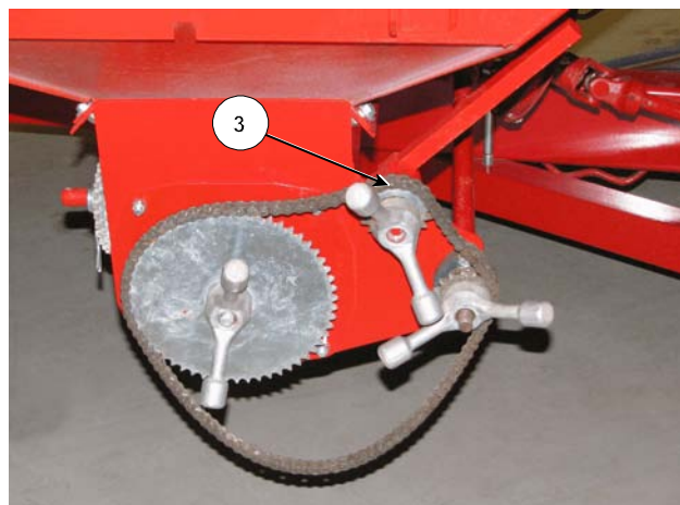
Loosen and Remove the Drive Chain
