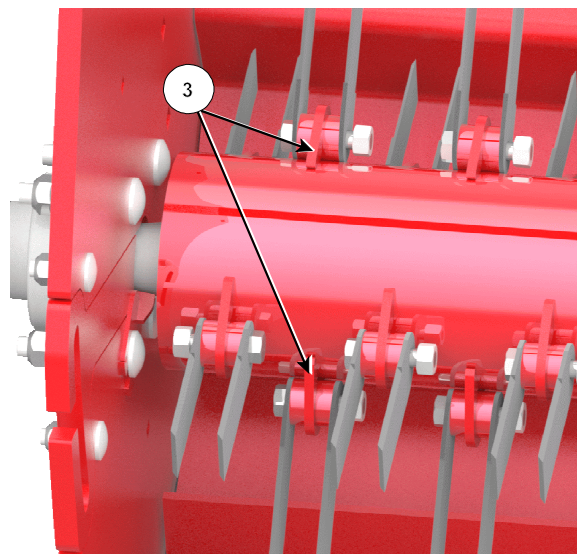
Replace Knife Set & Opposite Set
