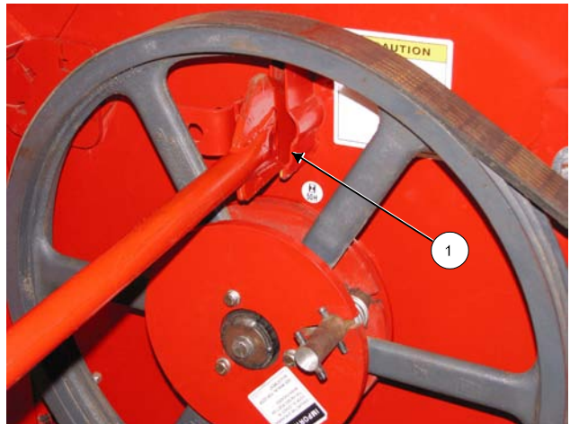
Twine Cutter Access
